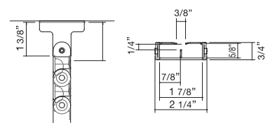
Cable Guard Dimensions
