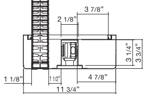
Wiring Duct Dimensions
