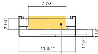
Wiring Duct Joint Part Dimensions
